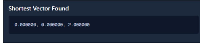
Fig. 13. The SVP we gained, which only shown in the final step of the BKZ process
